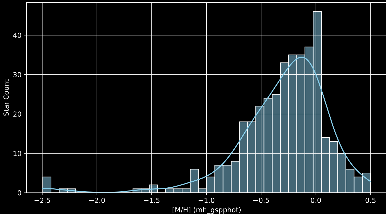
APOGEE DR17 Field: [180+75 [M/H] (mh_gspphot) (n= 391)
