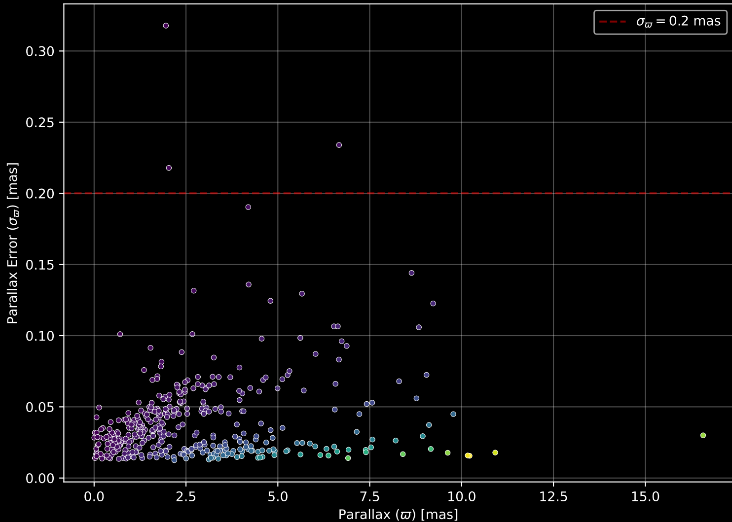
APOGEE DR17 Field: [180+75] Parallax Quality (n= 398)
