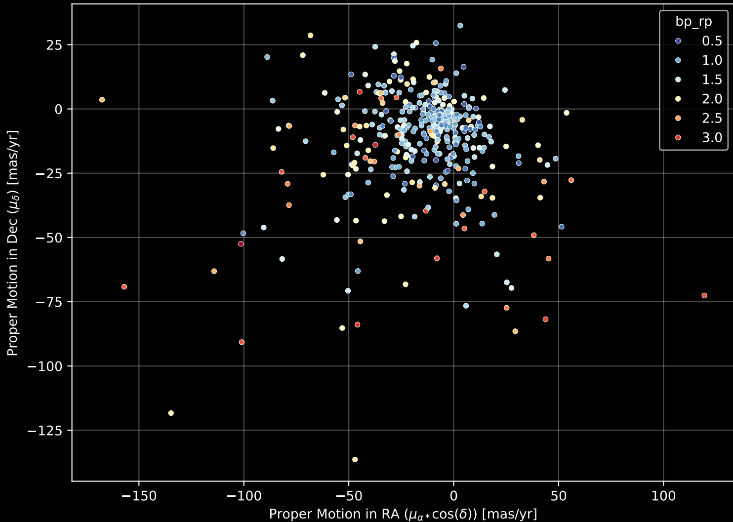
APOGEE DR17 Field: [180+75] Proper Motion Diagram (n= 398)
