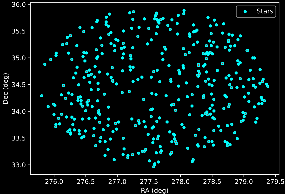
APOGEE DR17 Field: [180+75] Proper Motion Vectors for Gaia Star Field (n= 398)
