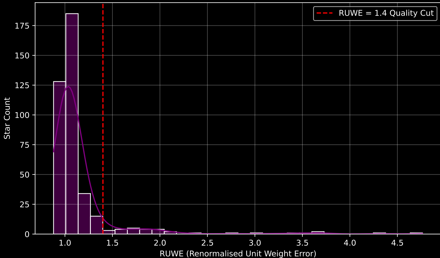
GAPOGEE DR17 Field [180+75] RUWE Distribution (n= 393)
