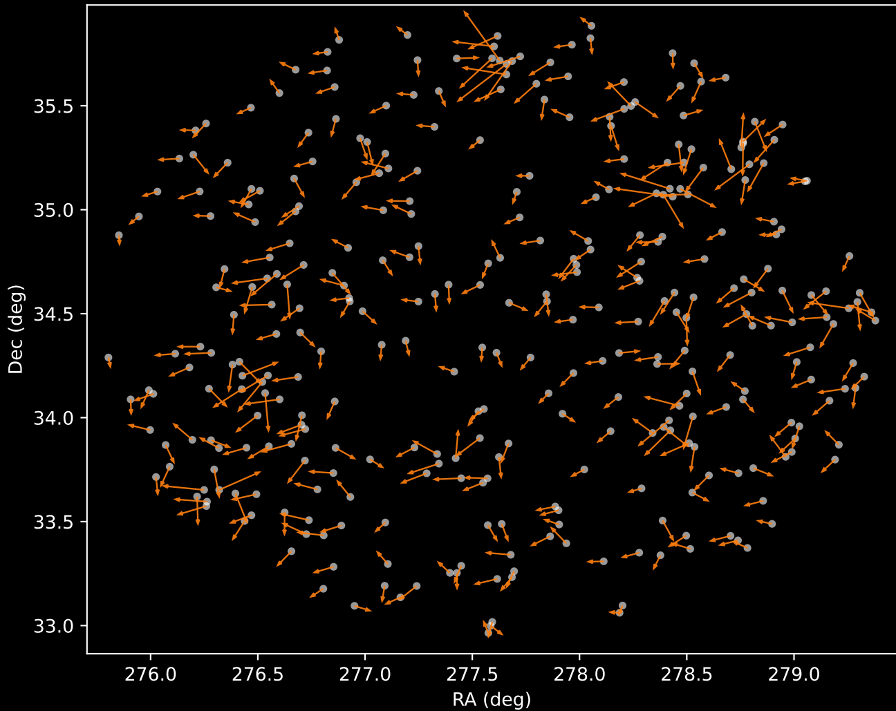
APOGEE DR17 Cluster 2 Proper Motion Vectors (n=337)
