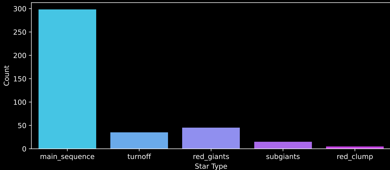
APOGEE DR17 Field: [180+75] Count plot of Star Type
